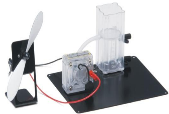
Generation of Electricity with Fuel Cell (H 2 /Air)
