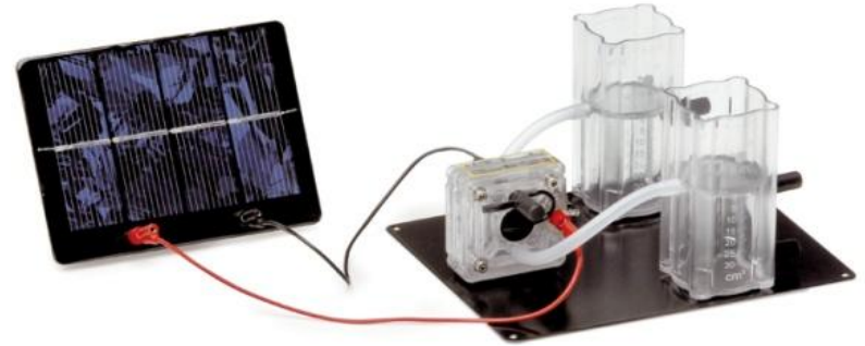
Production of Hydrogen & Oxygen with Electrolyser
