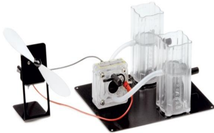
Generation of Electricity with Fuel Cell (H 2 /O 2 )
